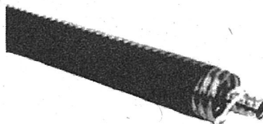
3-1/8" HELIFLEX® Air Dielectric Coaxial Cable
